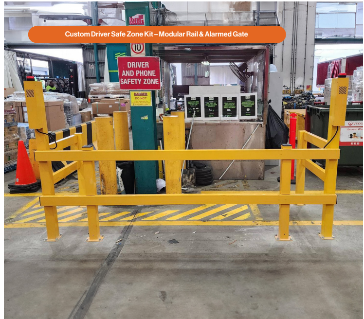
Custom Driver Safe Zone Kit - Modular Rail & Alarmed Gate
