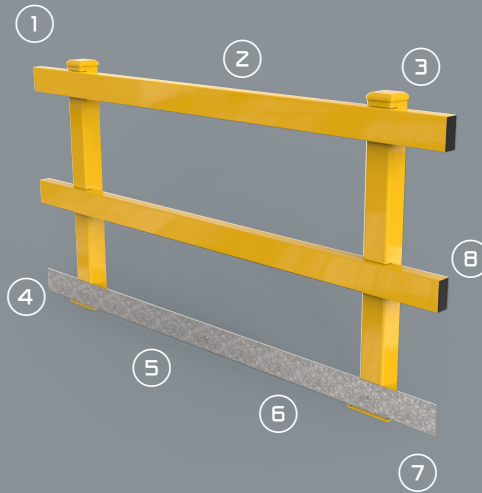
Pictured: 2m 'Recessed Rail' with Kick Plate
