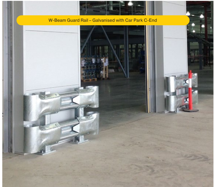
W-Beam Guard Rail - Galvanised Surface Mounted with Internal Corners and Car Park C-End
